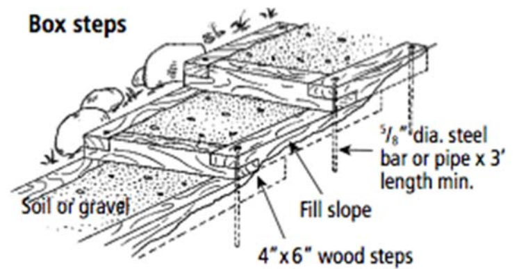
Box Stair Options
