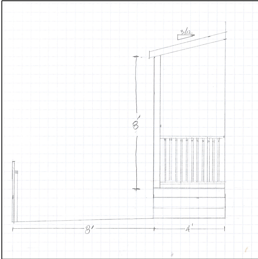
West Elevation
