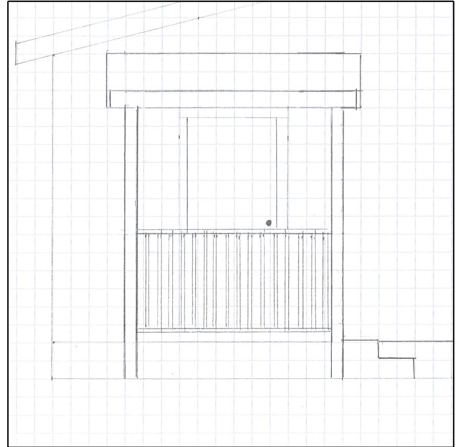
North Elevation
