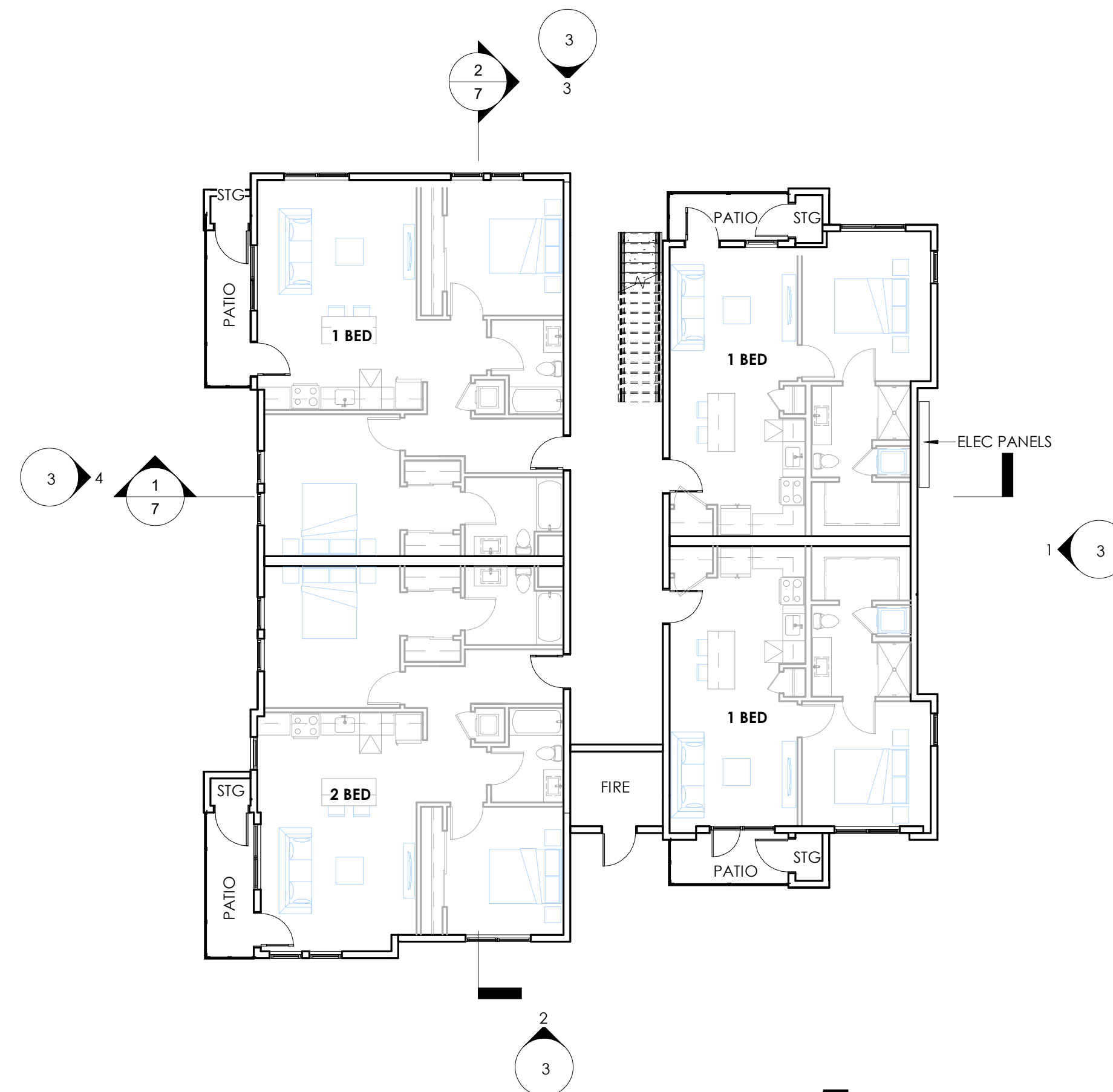
BLDG 1 - LEVEL 1
