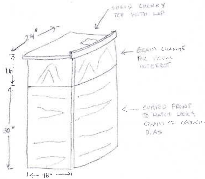
FORT BRAGG TOWN HALL LECTERN SKETCH
